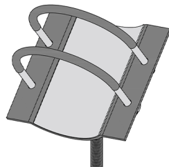
UES U-BOLT ELBOW SUPPORT
