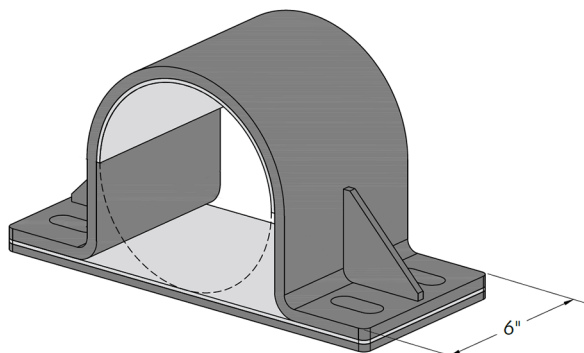
For pipes sized 4" through 24" Shown with optional liners and slotted holes.
